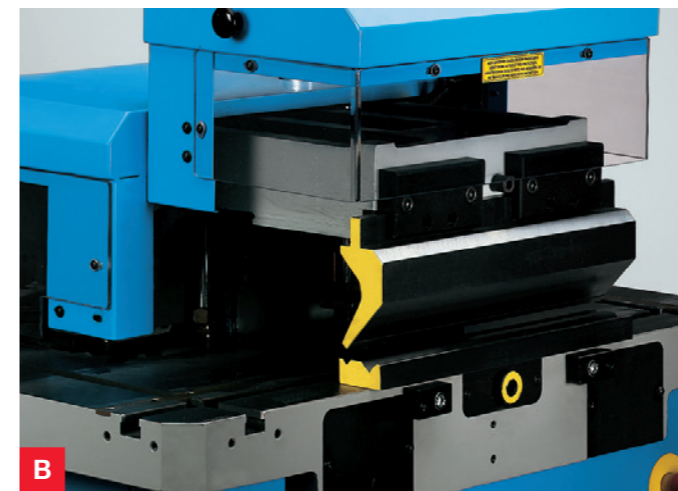
Press brake tooling Bends metal up to 415 mm long (5 mm thick) without disrupting your larger press brake.
