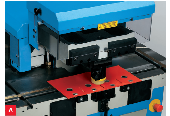
Tool holder for punching Accepts conventional Trumpf style round, square, & shaped tools up to 50 mm in diameter.
