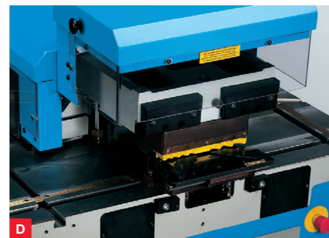
Radiusing Unit Various pre-sets for instant corner radiusing (3-15 mm radii) in material up to 6 mm thick.
