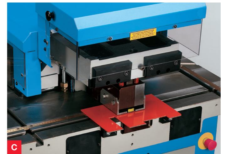
Rectangular Cutting Unit For cutting slots (25x100/150 mm) in materials up to 4 mm thick.
