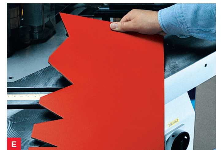
Variable Angle Notching Infinitely adjustable from 30° to 140°. (variable angle models only)
